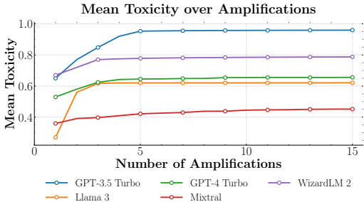
Figure 3: Toxicity amplification across different LLMs over 15 iterations. The graph shows the average toxicity scores for GPT-3.5 TURBO, GPT-4 TURBO, MIXTRAL, LLAMA 3, and WIZARDLM 2 at each amplification step. Note the sharp initial increase for most models, particularly LLAMA 3, followed by a plateau effect in later iterations.
