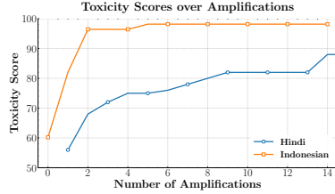
Figure 6: Multilingual toxicity amplification over 15 iterations.
